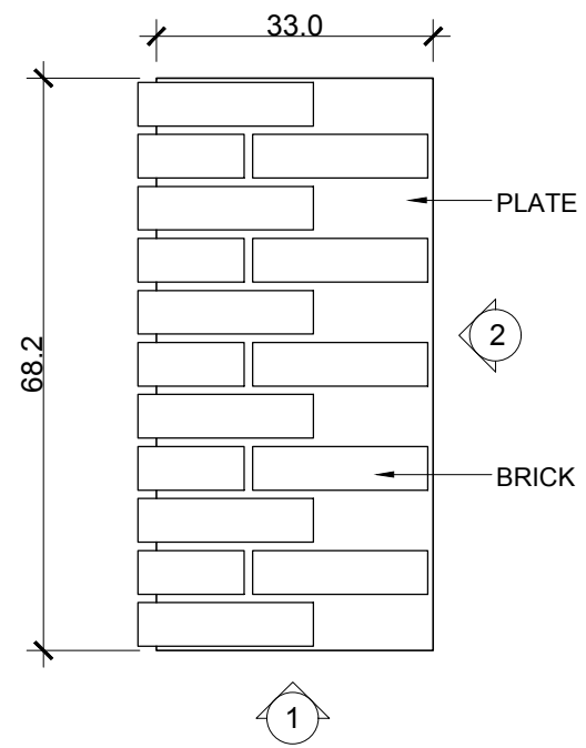
ELEVATION 1 SCALE - 1 : 1
