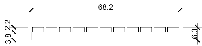
ELEVATION 2 SCALE - 1 : 1
