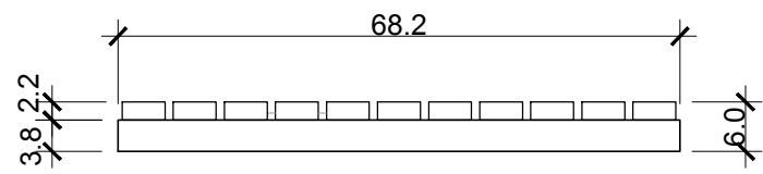
ELEVATION 2 SCALE - 1 : 1
