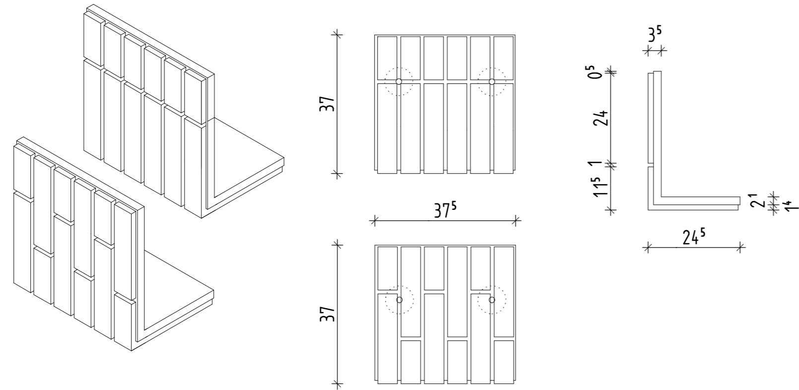
ETICS/WDVS SYSTEM KESS DF (370x245mm) STURZECKE ST8
