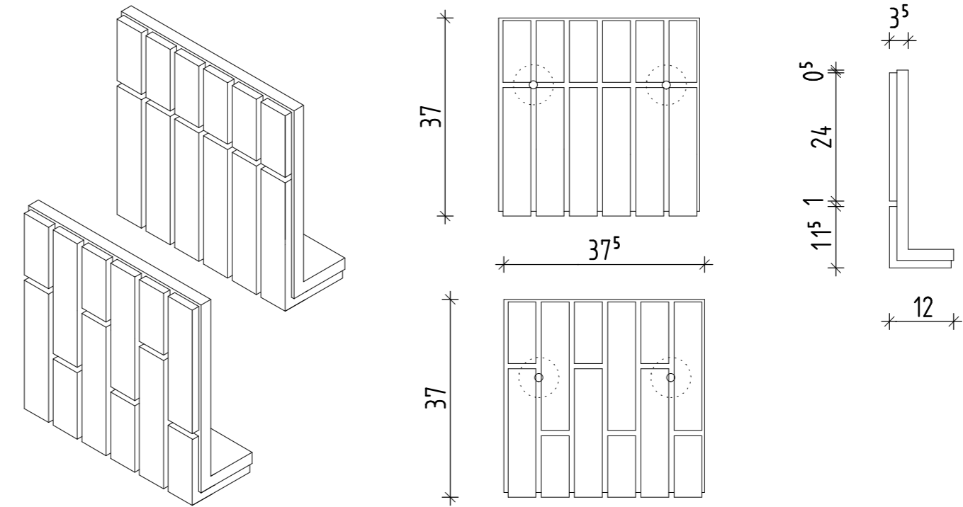
ETICS/WDVS SYSTEM KESS DF (370x370mm) STURZECKE ST9
