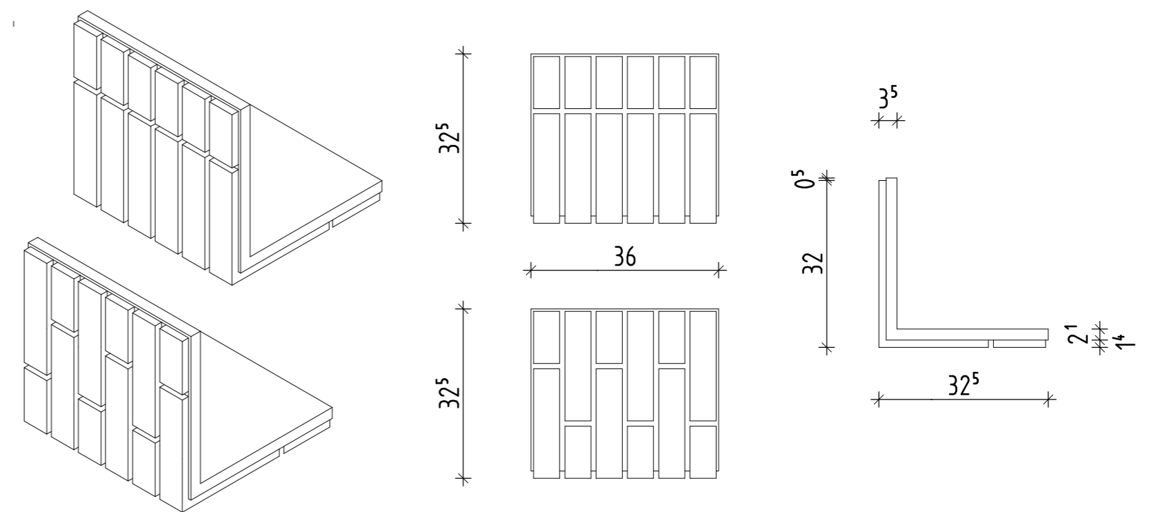
ETICS/WDVS SYSTEM KESS WF210 (325x325mm) STURZECKE ST9
