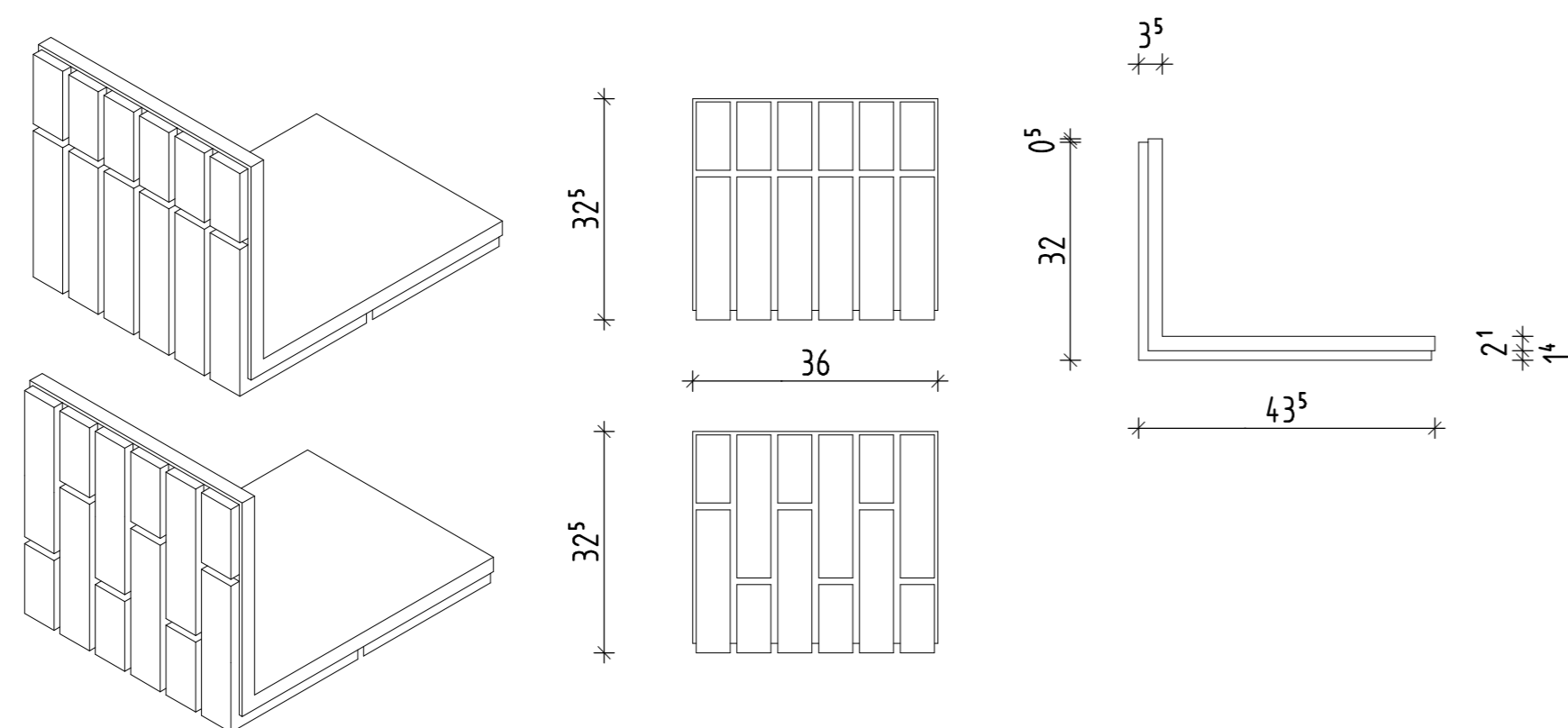
ETICS/WDVS SYSTEM KESS WF210 (325x435mm) STURZECKE ST10
