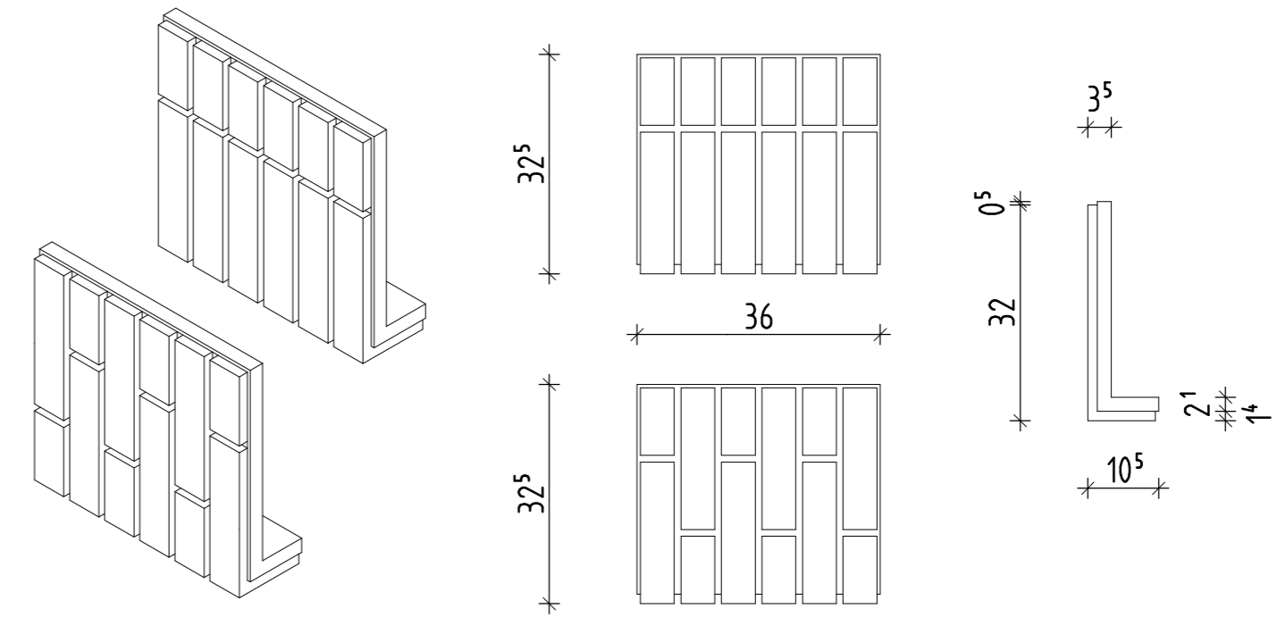
ETICS/WDVS SYSTEM KESS WF210 (325x105mm) STURZECKE ST7
