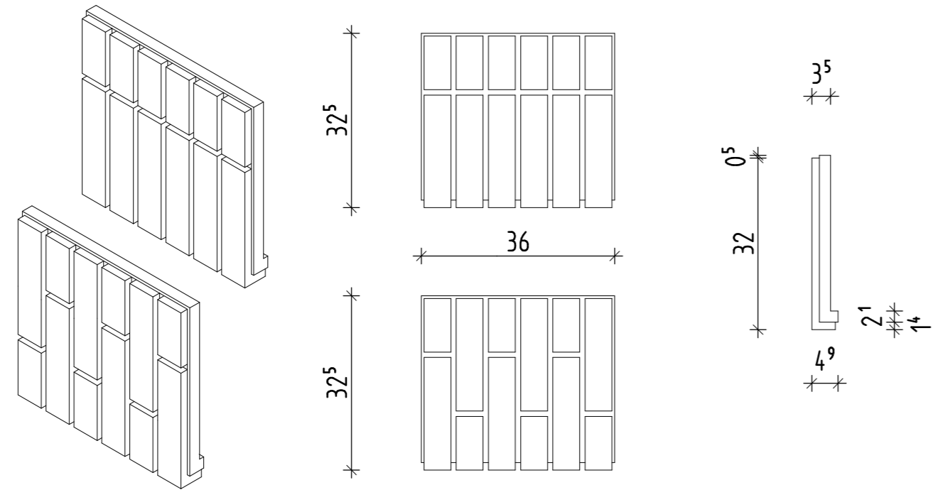
ETICS/WDVS SYSTEM KESS WF210 (325x49mm) STURZECKE ST6
